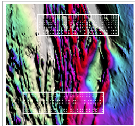
Magnetics using HSI enhancement
