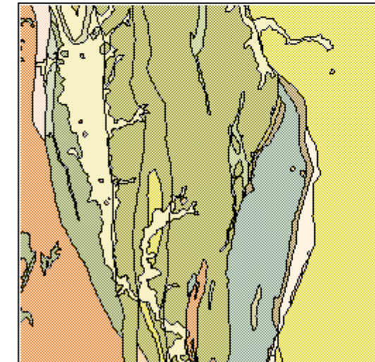
250k geology overlaying magnetics
